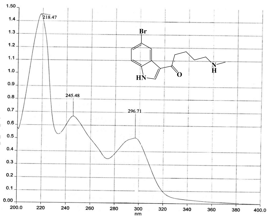
UV SPECTRUM
