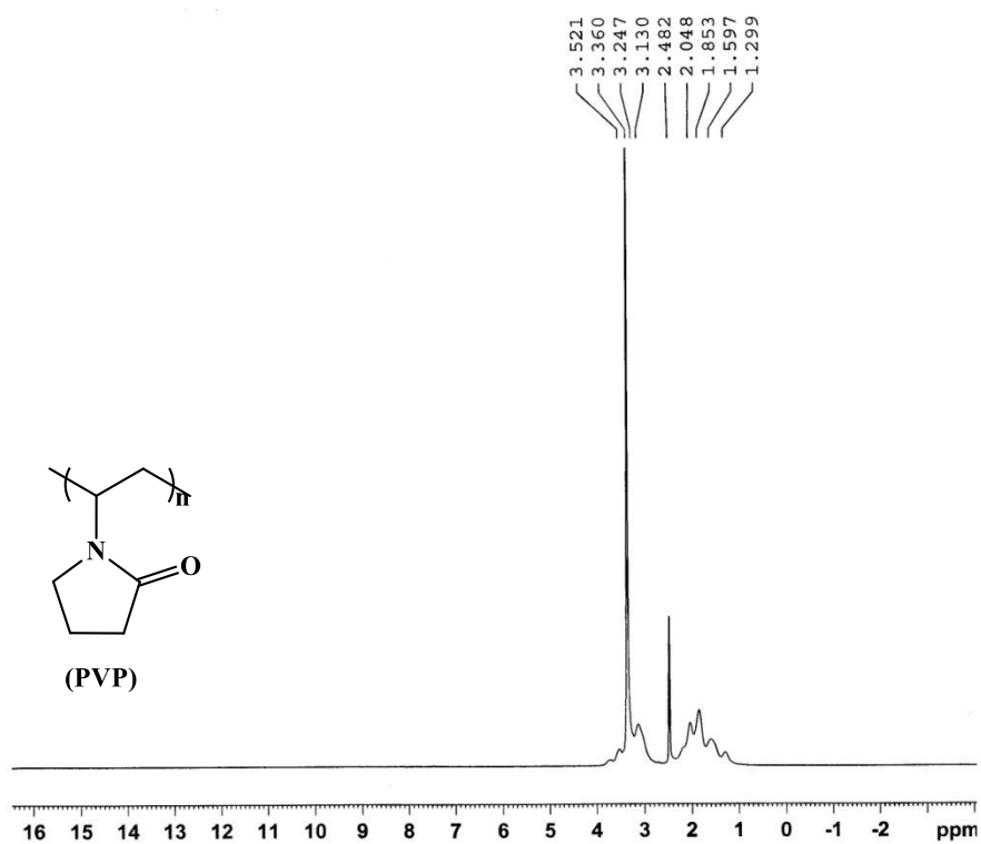
1 H-NMR SPECTRUM
