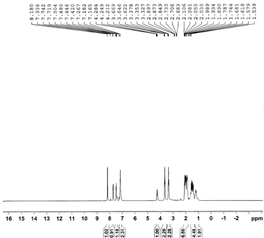
1 H-NMR SPECTRUM
