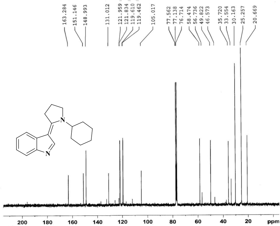
13 C-NMR SPECTRUM
