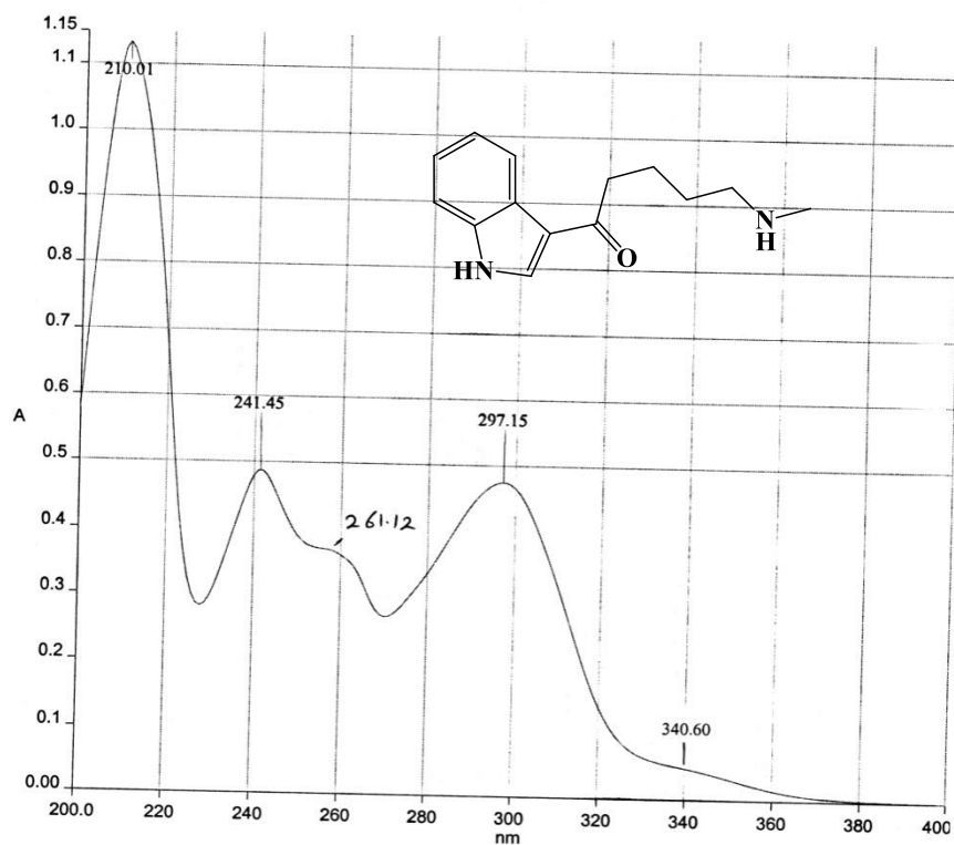
UV SPECTRUM
