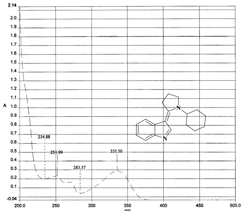
UV SPECTRUM
