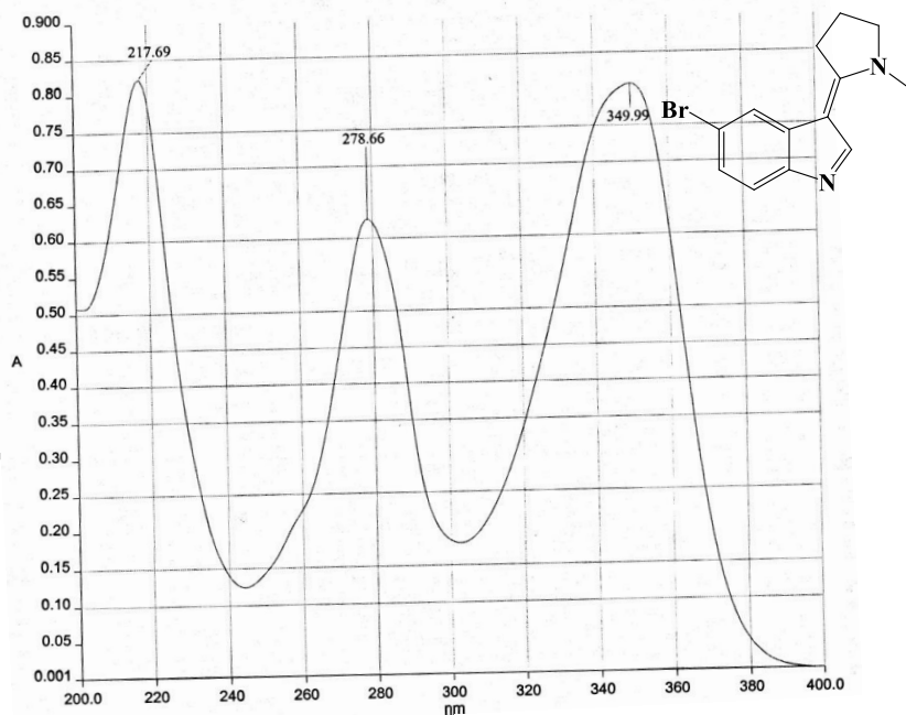
UV SPECTRUM
