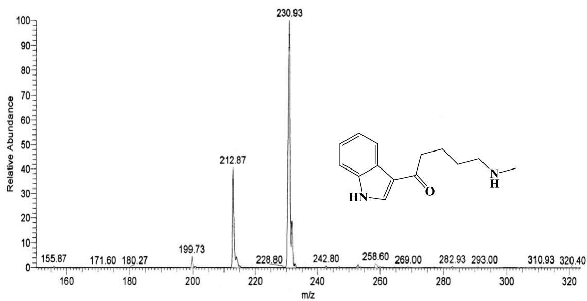
GC-MASS SPECTRUM
