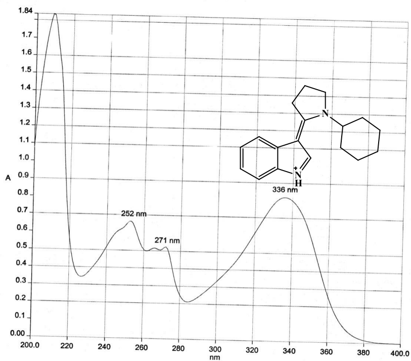
UV SPECTRUM
