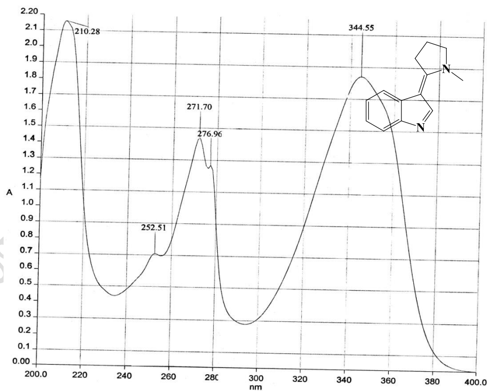
UV SPECTRUM
