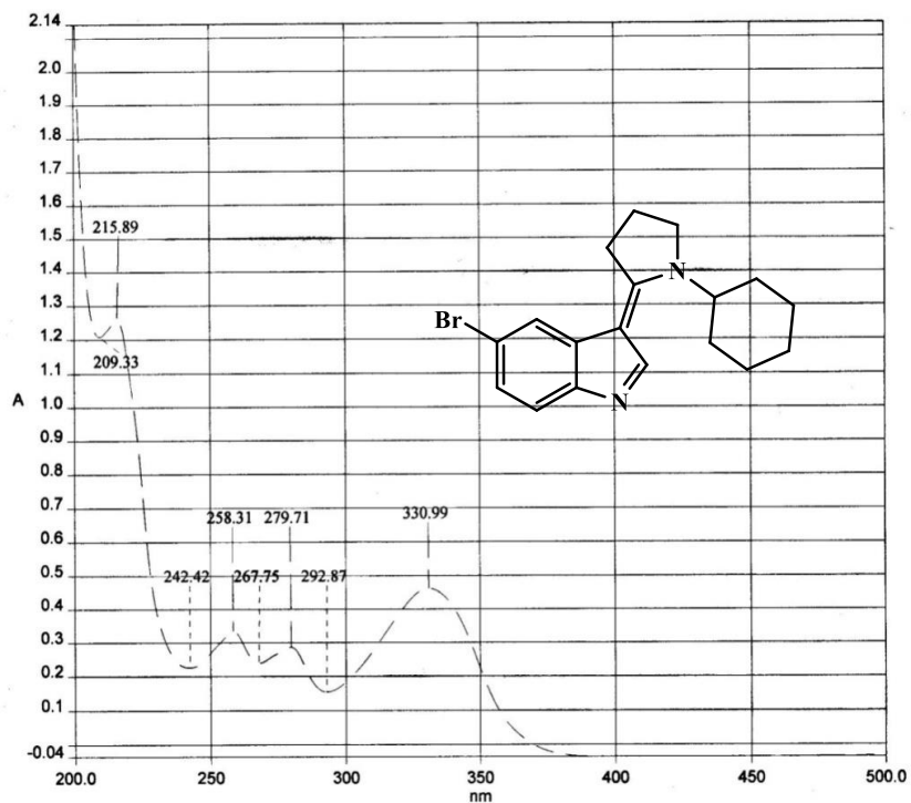
UV SPECTRUM
