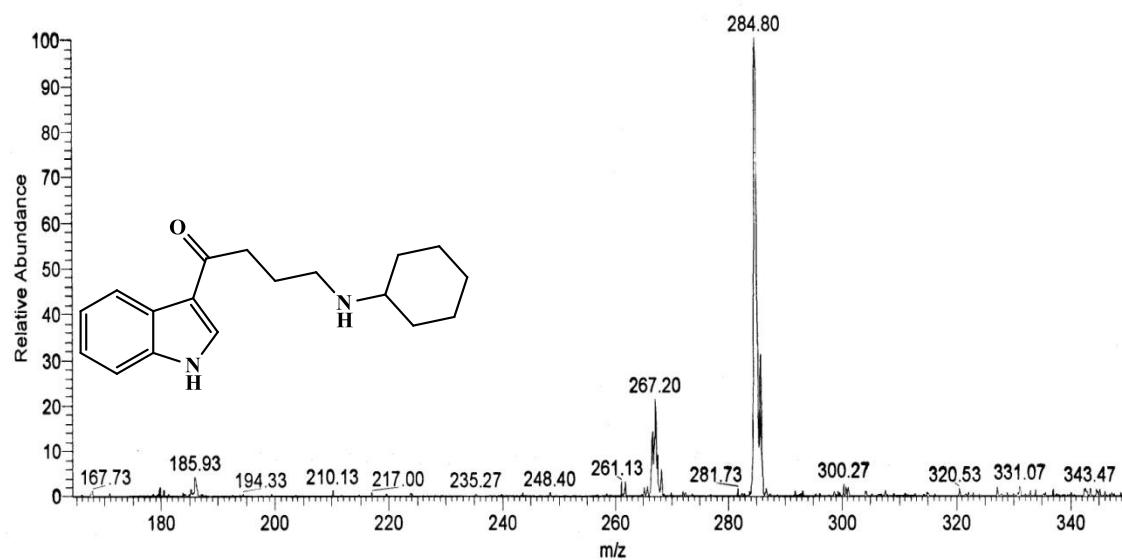
GC-MASS SPECTRUM
