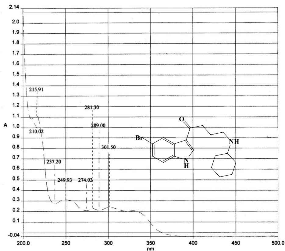
UV SPECTRUM
