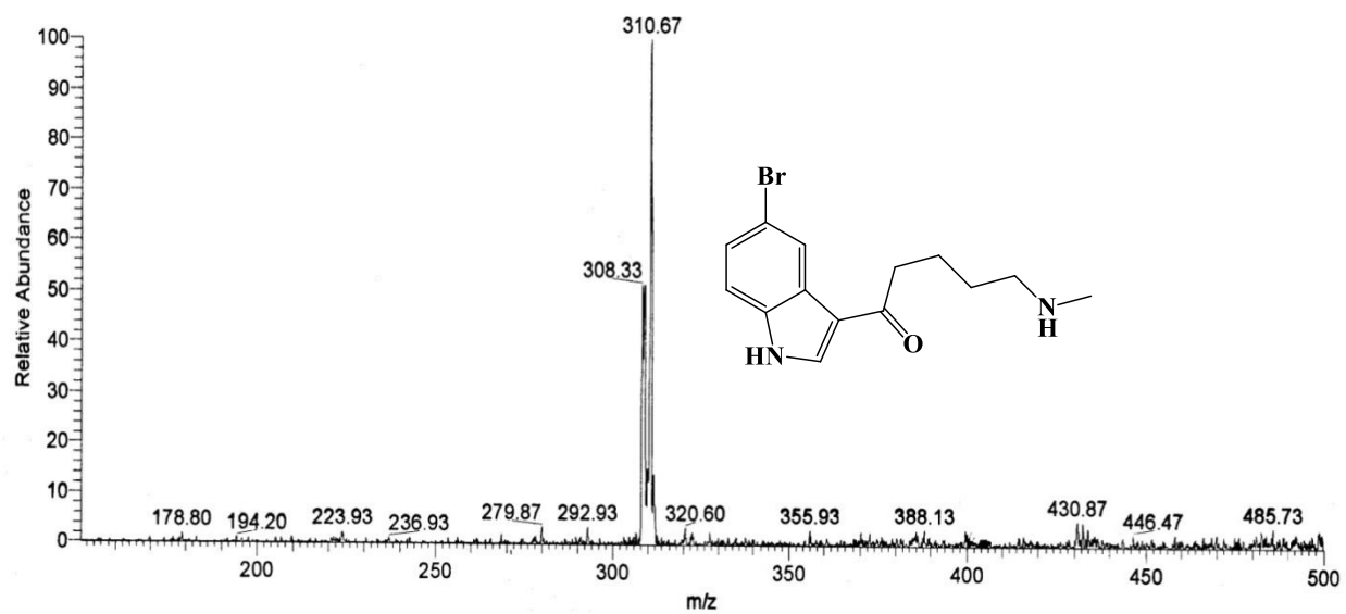
GC-MASS SPECTRUM
