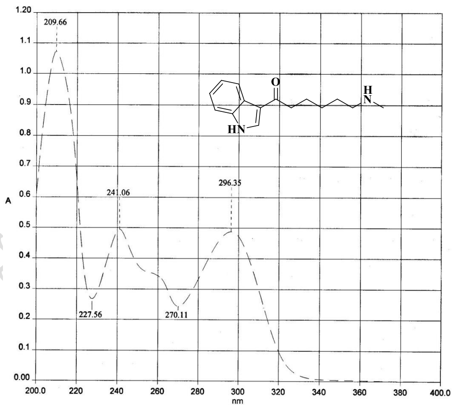
UV SPECTRUM
