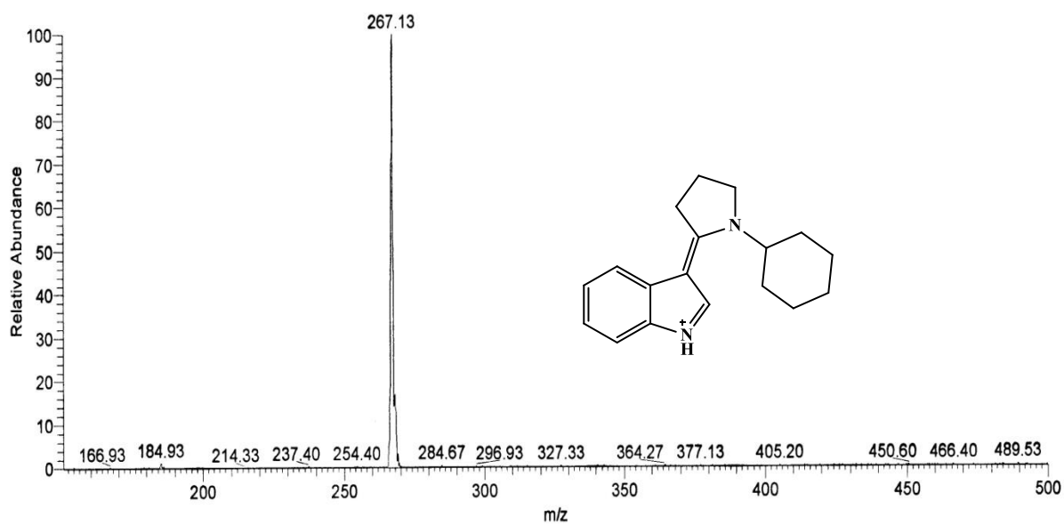
GC-MASS SPECTRUM
