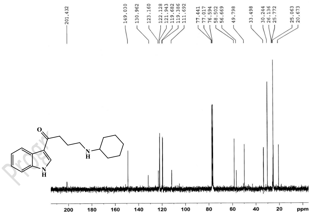
13 C-NMR SPECTRUM
