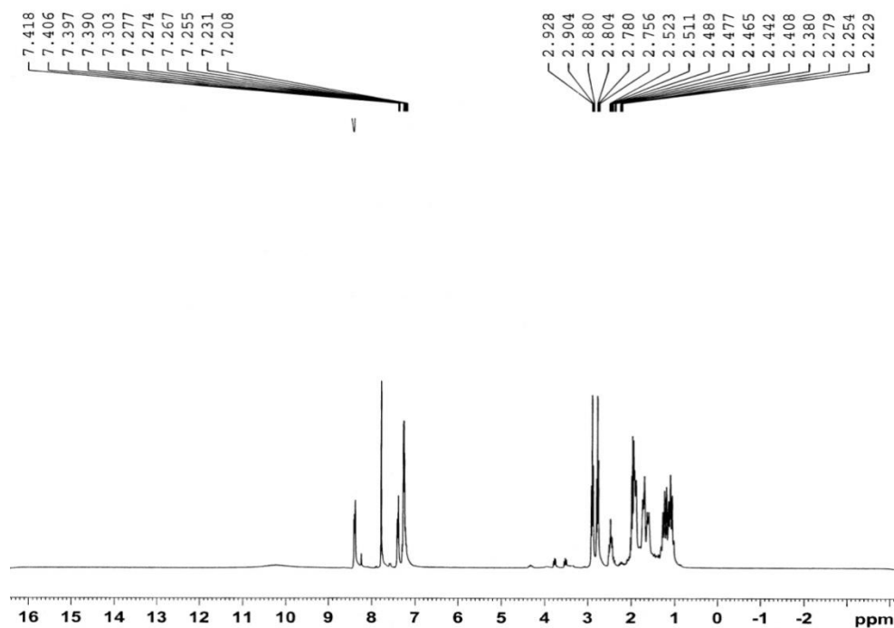
1 H-NMR SPECTRUM
